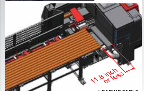
LOADING TABLE
